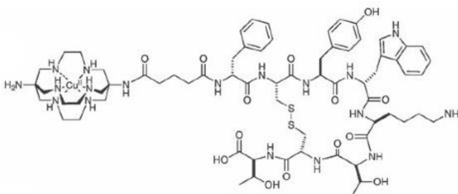
Fig. 5. Chemical structure of ^{64}\text{Cu} -SARTATE.
