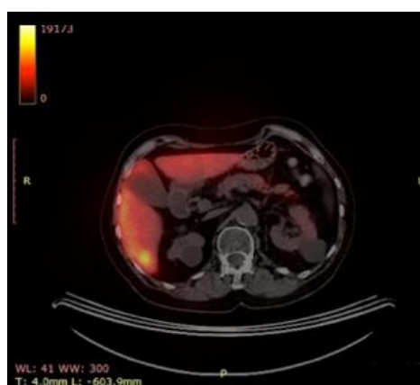
Fig. 3. Uptake of ^{64}\text{Cu}^{2+} in liver cancer.
